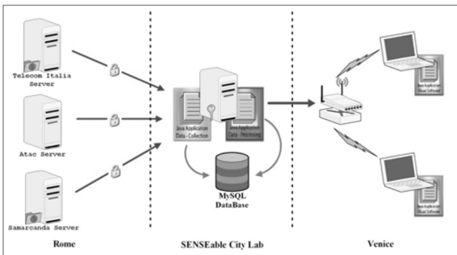
Figure 1. Schematic of the data collection, transfer and processing
