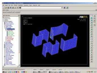
Fig. 11 Tsunami Safe(r) House: elastic deformation under load normal to coastline
