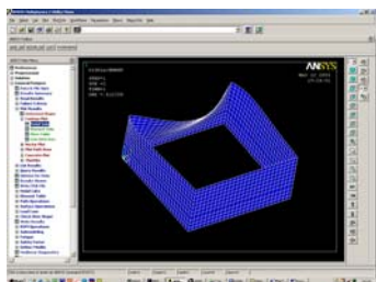
Fig. 10 Typical dwelling: elastic deformation under horizontal load normal to coastline
