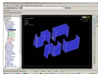
Fig. 12 Tsunami Safe(r) House: elastic deformation under load parallel to coastline
