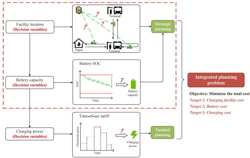
Fig. 3. Overview of the integrated optimization problem.
