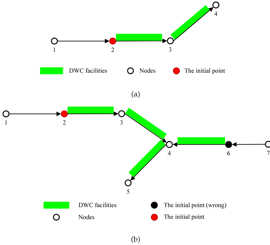
Fig. 4. Illustrations of the connections of DWC facilities.
